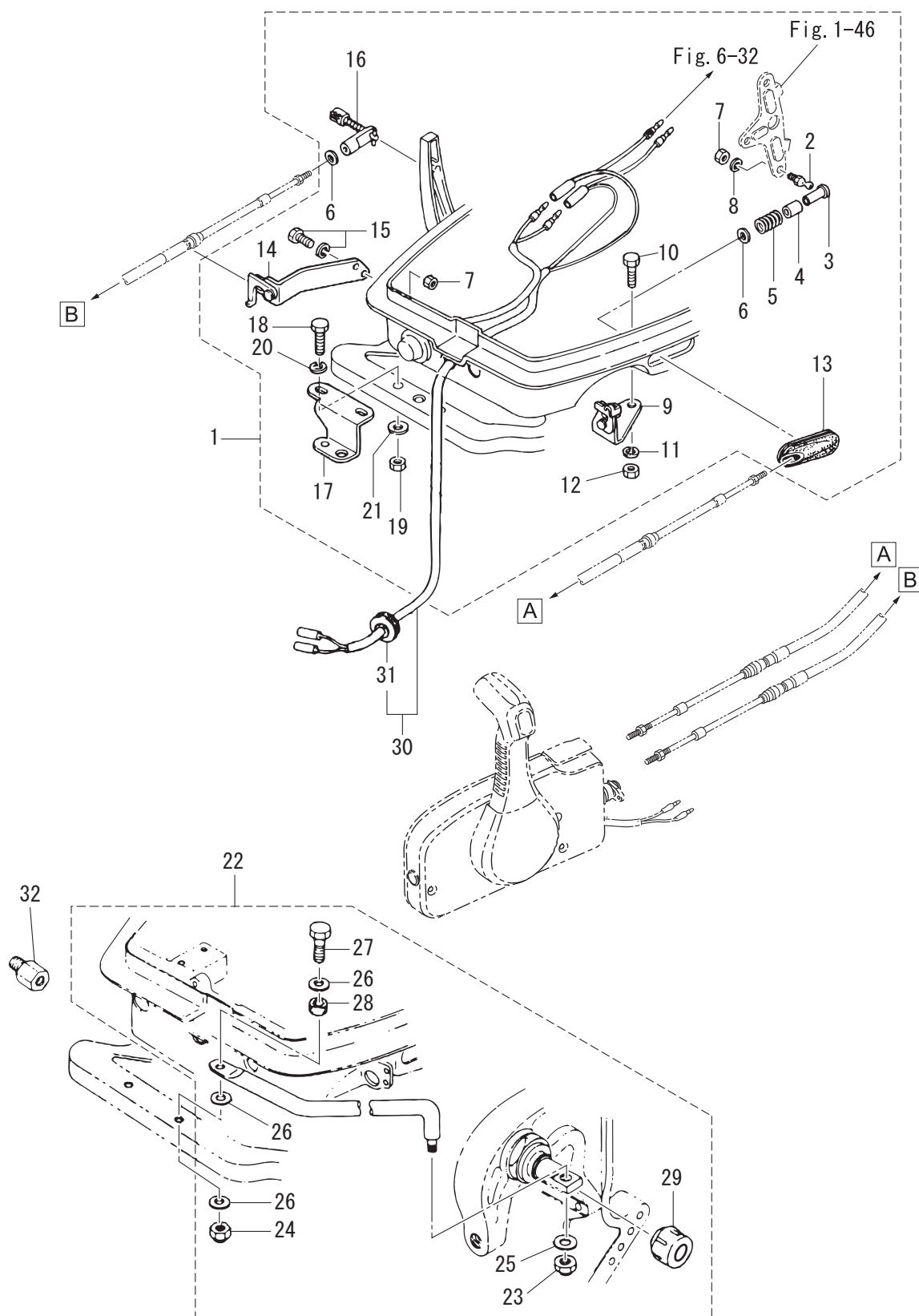
REMOTE CONTROL PARTS
